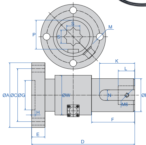
dimension drawing
